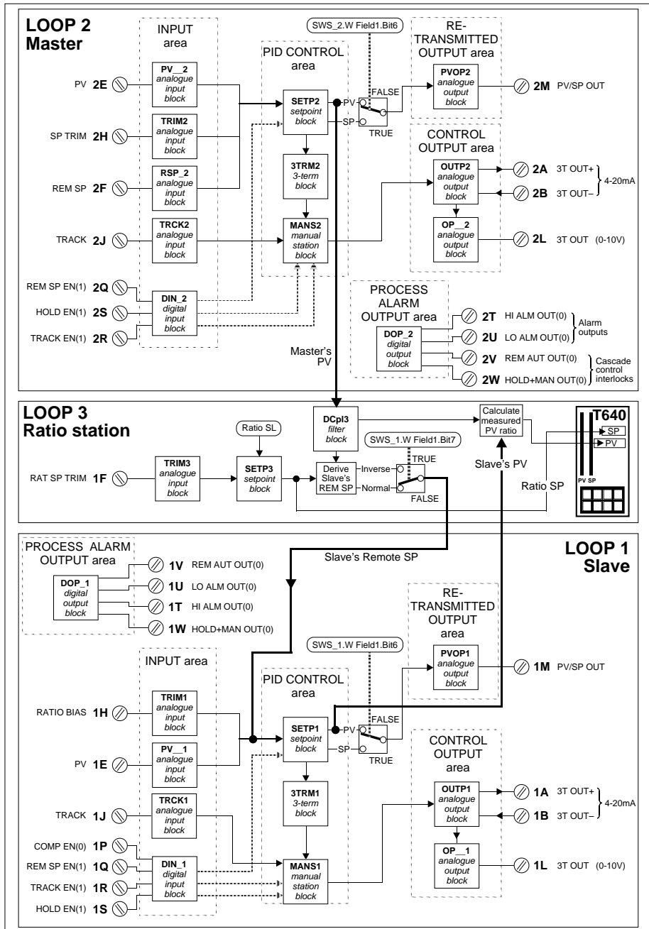
Figure 5-9 Strategy #4 schematic
