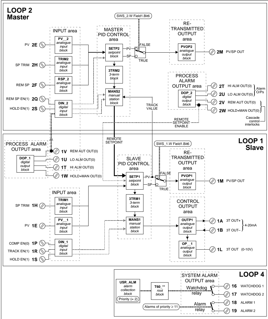
Figure 5-7 Strategy #3 schematic
